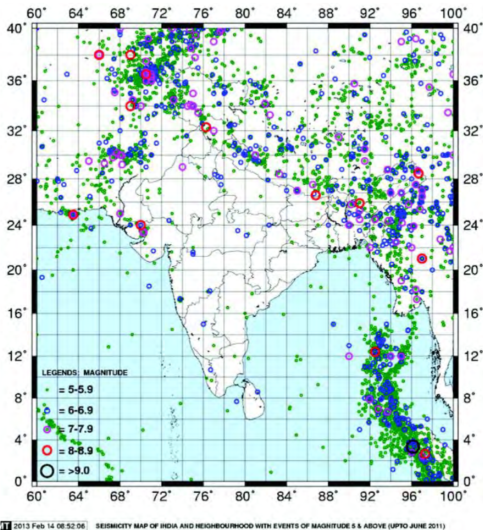
Fig. 6: Seismicity map of India ( M \geq 5.0 ) and neighborhood for the period upto June, 2011
