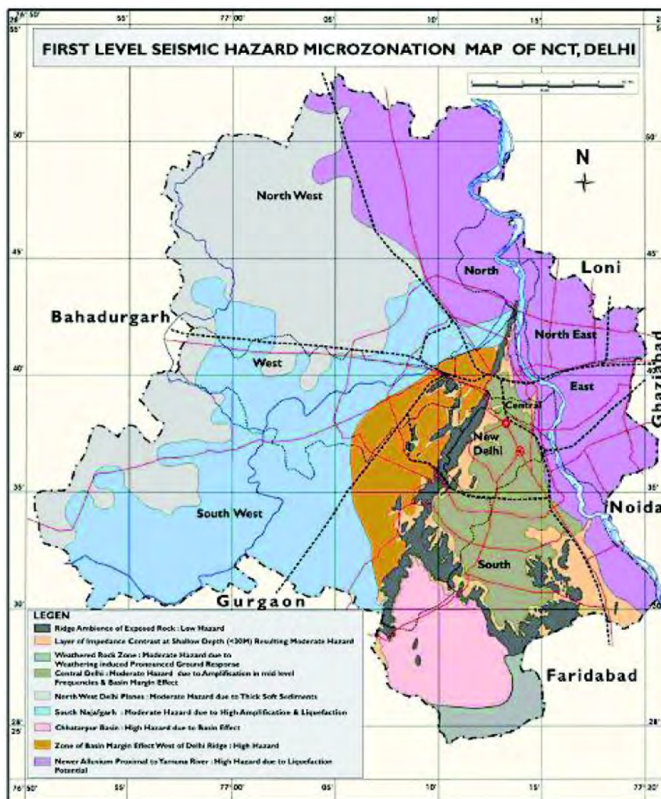
Fig. 4: Seismic microzonation map of NCT, Delhi on 1:50,000 scale
