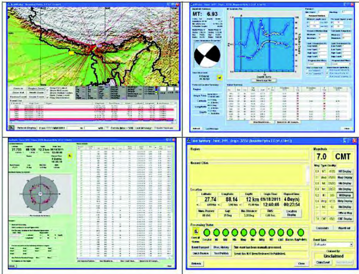
Fig. 2: Real time earthquake products generated by the RTSMN system for the Sikkim earthquake of 18 th September, 2011
