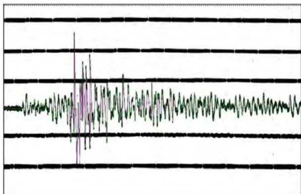
Fig. 7: Digitized seismogram superimposed on the original analog record of Anjar, Gujarat earthquake (M:7.0) of 21.7.1956 recorded at Shillong
