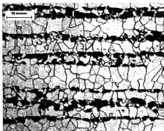
Fig. 3. A wrought 1018 steel slow cooled from 900 °C to room temperature. Deformation direction is horizontal (Nital etch, 240x)
