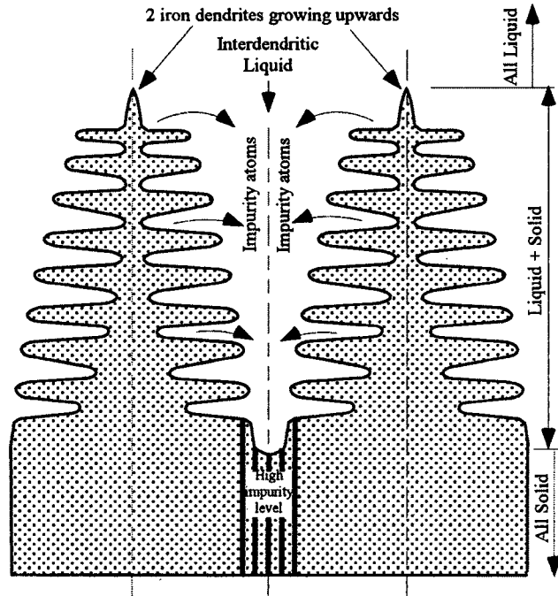
Fig. 5. Neighboring iron dendrites growing into the liquid.
