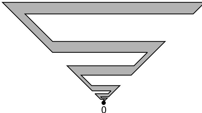
Figure 9: A ‘fattened’ Jordan arc repeatedly crossing a triangle
