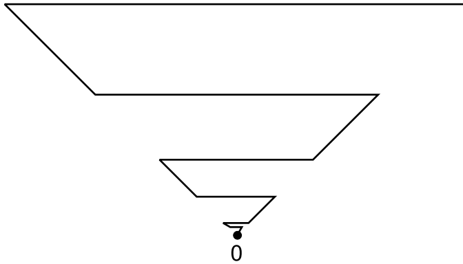
Figure 7: A Jordan arc repeatedly crossing a triangle
