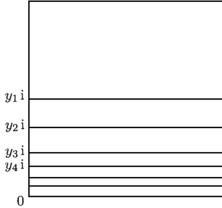
Figure 5: A square crossed by lines
