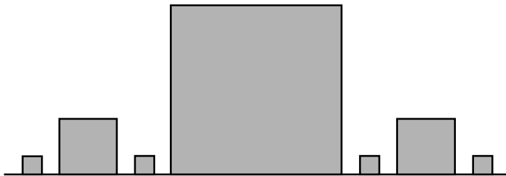
Figure 2: The Cantor set with squares attached
