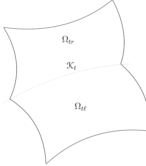
Figure 2: Figure is drawn in 3 space dimensions. Kink \mathcal{K}_t (shown with dotted lines) on \Omega_t = \Omega_{tr} \cup \Omega_{tl} .
