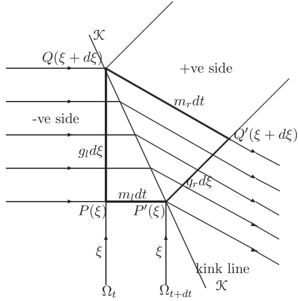
Figure 1: A 2-D analog of the kink phenomenon in (x_1, x_2) -plane corresponding to a shock moving down on \Omega_t in negative \xi -direction, here d\xi > 0 . In this case \Omega_t is a curve consisting of two lines meeting at a kink \mathcal{K}_t , which is a point Q on the ray corresponding to \xi + d\xi . \Omega_{t+dt} is a curve with kink at P' on the ray corresponding to \xi . The kink surface \mathcal{K} becomes a kink line passing through the points Q and P' .
