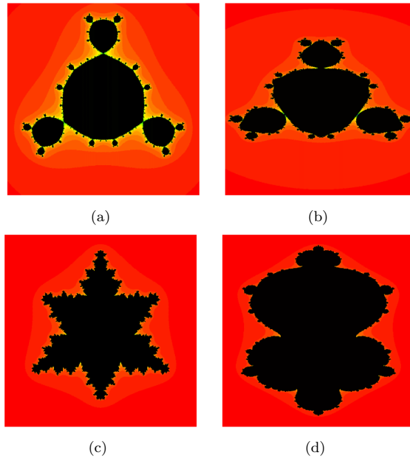
Figure 1: Julia set for Q_c(z) = z^3 + (3/2)z + c and c = 1.75i in (a) Jungck and (b)-(d) Jungck-CR orbit
