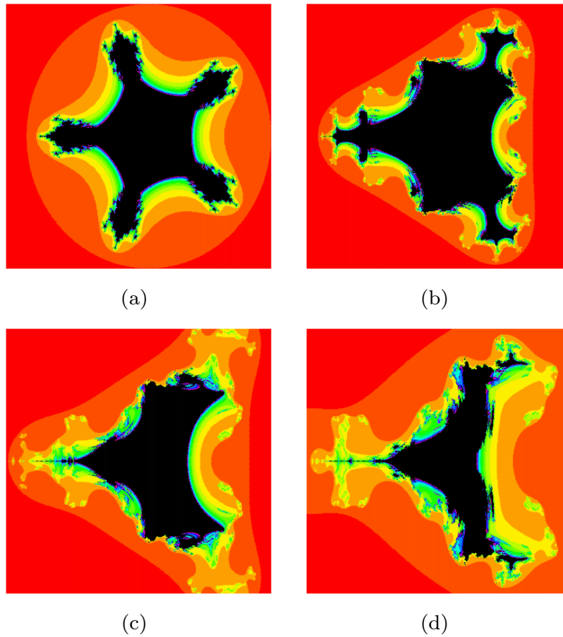
Figure 5: Multicorn set for Q_c^*(z) = \bar{z}^4 + 3\bar{z} + c in (a) Jungck and (b)-(d) Jungck-CR orbit
