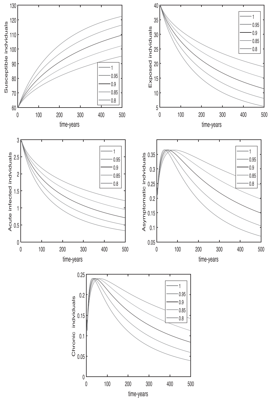
Fig. 1 Numerical solutions of Model (7)–(8) for \theta = 0.09 , and various dimensions ( \gamma )
