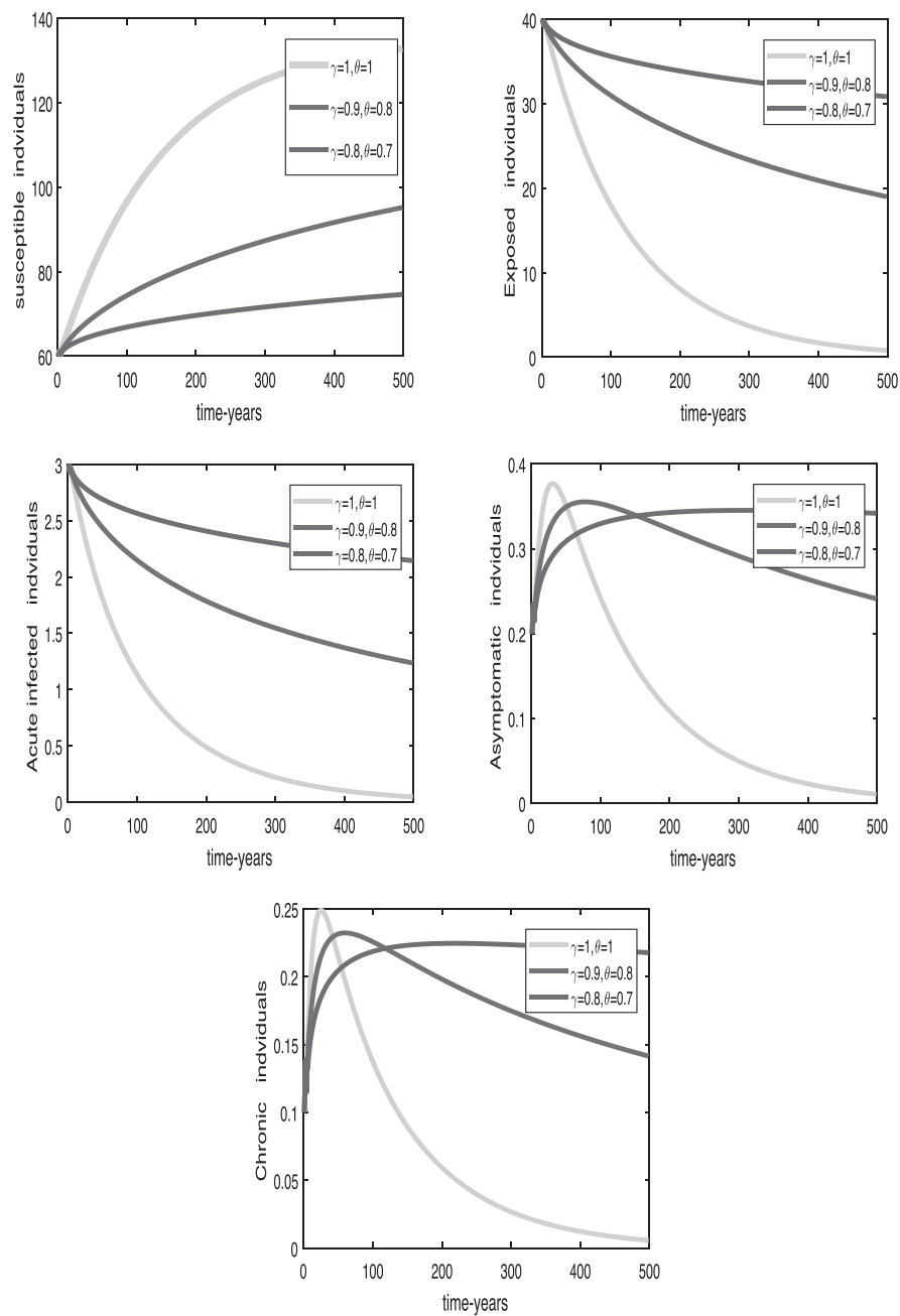
Fig. 3 Numerical solutions of Model (7)–(8) for difference \theta = 1, 0.8, 0.7 , and \gamma = 1, 0.9, 0.8 , respectively
