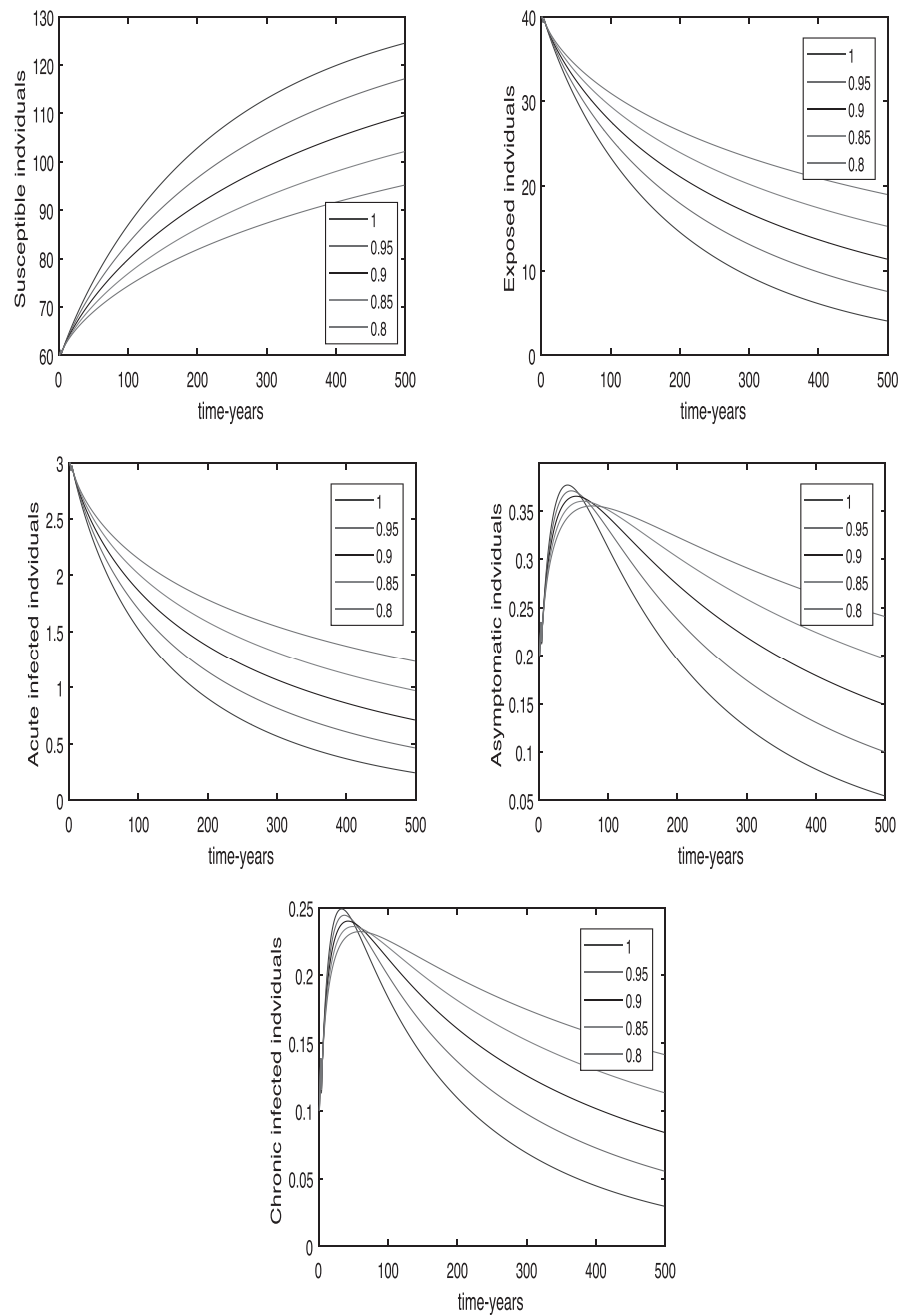
Fig. 2 Numerical solutions of Model (7)–(8) for \gamma = 0.09 , and various ( \theta )
