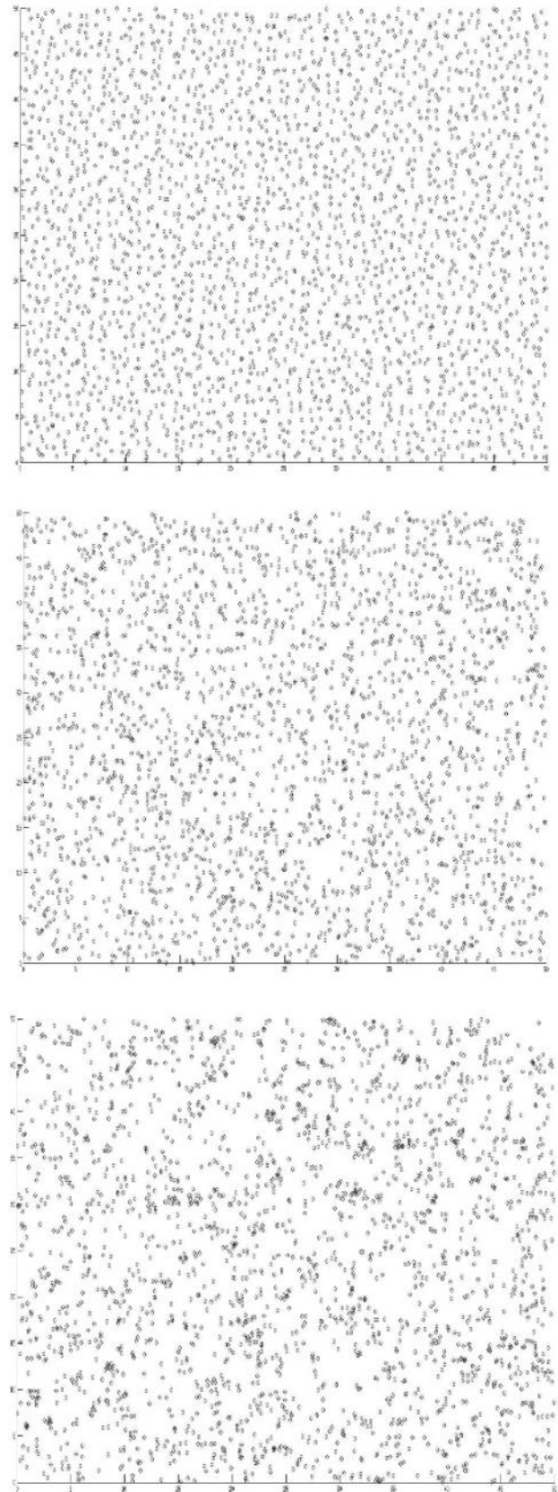
Fig. 1: Hypergeometric perturbed lattice, Poisson point process and Negative binomial perturbed lattice
