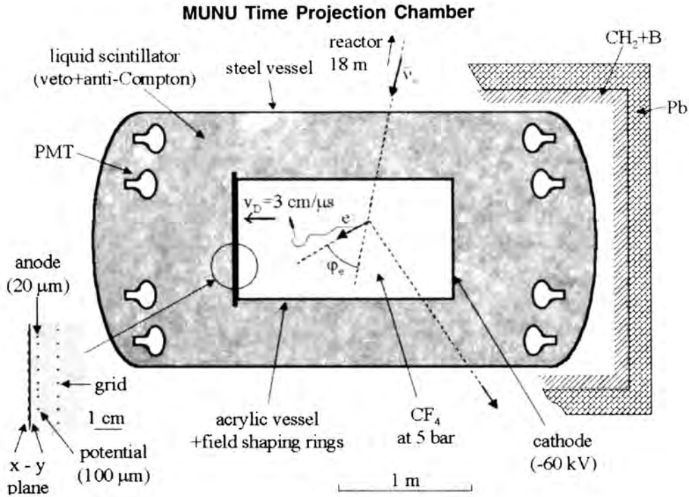
Fig. 7 A schematic view of the arrangement of the MUNU experiment. It measures the recoil energy and angle of the electron following antineutrino-electron elastic scattering
