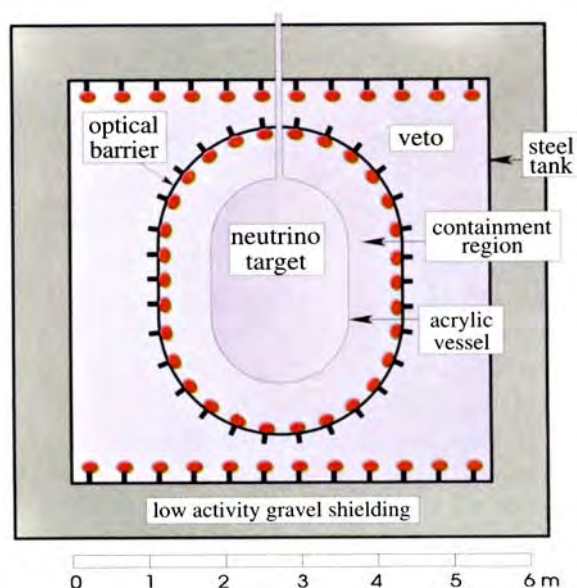
Fig. 1 The CHOOZ detector. The neutrino target consists of a 5 ton 0.09% Gd loaded liquid scintillator. The containment region consists of 17 ton liquid scintillator. Surrounding these is a 90 ton active muon veto shield. Figure taken from ref. [13].
