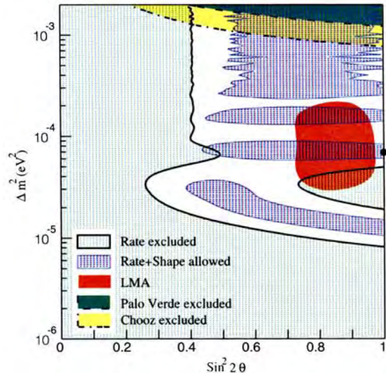
Fig. 6 Excluded and allowed regions in the \delta (shown as \Delta m^2 in the figure) and \sin^2 2\theta from the various reactor based antineutrino oscillation experiments. The allowed LMA (large mixing angle) solution from the solar neutrino analysis is also indicated. The thick dot indicates the best fit to the KamLAND data. The 95% confidence level allowed regions from KamLAND are also shown. Figure taken from ref. [15]
