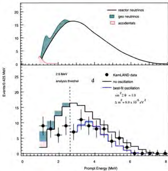
Fig. 5 Top: Expected 'prompt' energy spectrum due to antineutrinos from the reactor and background sources at the KamLAND detector. The lower panel shows a histogram of the measured 'prompt' spectrum along with one expected in the absence of oscillations. The lower histogram in the lower panel shows the best fit with oscillations.
