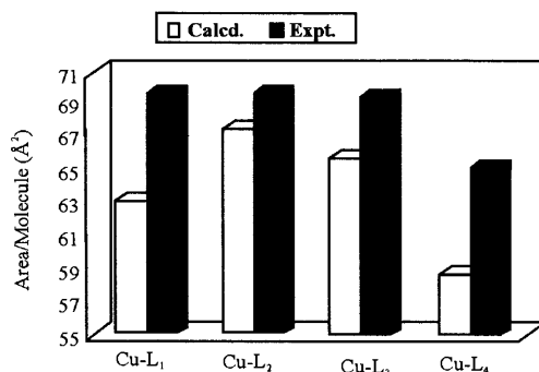
Fig. 8 Comparison of average area per molecule ( exp. & calcd.) of Cu(II)-complexed surfactants and stearic acid mixture (1:1) at 15 mN/m surface pressure
