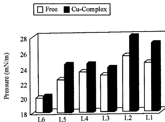
Fig. 4 Comparison of maximum surface pressure (mN/m) sustained by the amphiphiles
