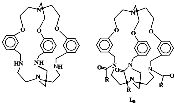
Fig. 1 Triple-tailed amphiphiles with two different cryptand headgroups
