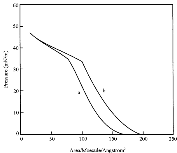
Fig. 9 Pressure-area isotherms for L 18 at 298 K (a) with pure water as sub-phase and (b) adenine (0.1 M) in pure water as sub-phase
