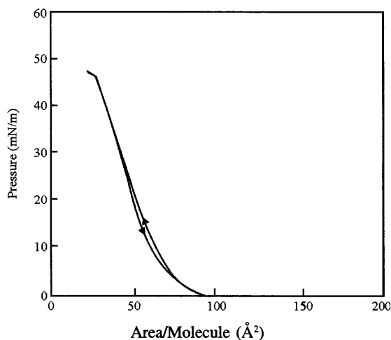
Fig. 6 Representative successive compression and expansion cycles ( hysteresis) with a monolayer of L_2
