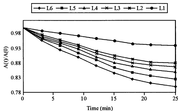
Fig. 5 Comparison of the stability of the monolayer at the air-water interface for the amphiphiles L 1 -L 6
