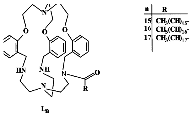
Fig. 2 Single-tailed amphiphiles
