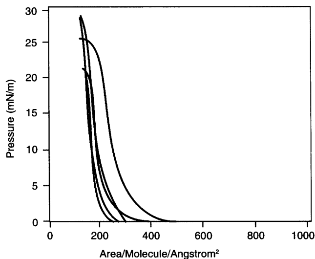
Fig. 3 Pressure-area isotherm for L 1 -L 6 (Series A amphiphiles) at 298 K. The Series B amphiphiles show similar isotherms
