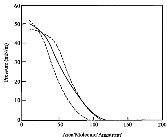
Fig. 7 Pressure-area isotherms for the single-tailed amphiphiles L_{15} - L_{17} at 298 K
