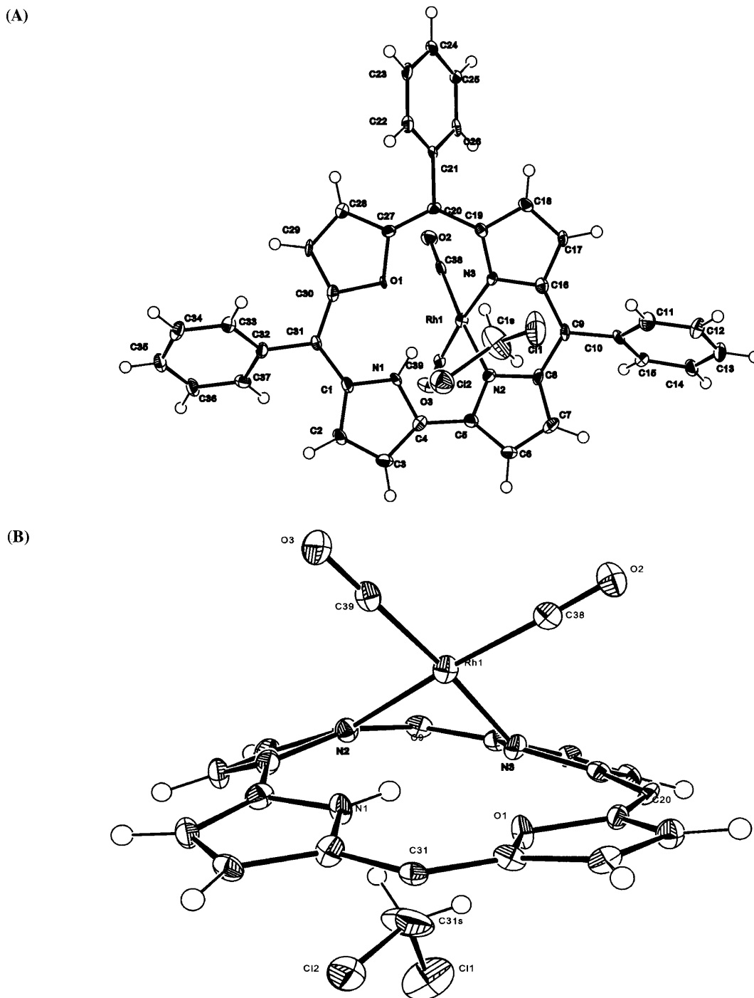
Fig. 1 ORTEP diagram for 3 (a) Top: Plane view (b) Bottom: Side view(phenyl rings are omitted for clarity) 13b
